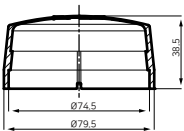
HP120
