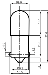
BA9S
