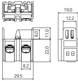
J2-10 / J2-01
