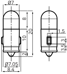
BA7S
