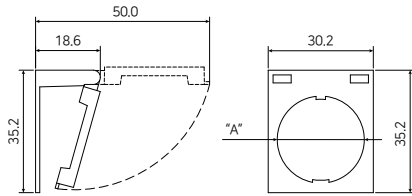
SC2, SC5
