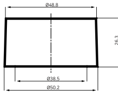
HP100
