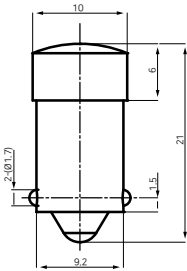
BA9S-B
