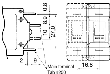
Rocker (Non-illuminated) Relay Trip (4-terminal)
