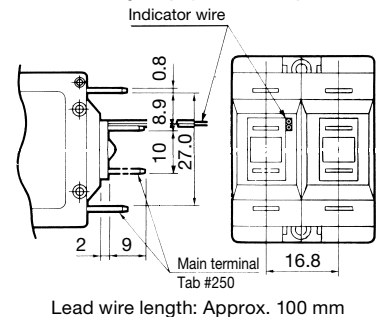
Illuminated Rocker (2-pole) Relay Trip (4-terminal)
