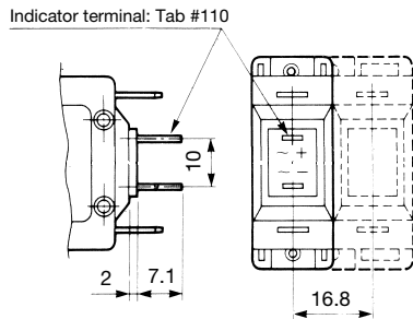
Illuminated Rocker (without auxiliary contact) Series Trip, Switch Only
