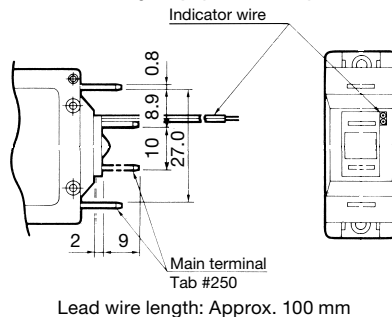
Illuminated Rocker (1-pole) Relay Trip (4-terminal)
