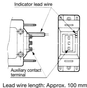
Illuminated Rocker (1-pole) Relay Trip (4-terminal)
