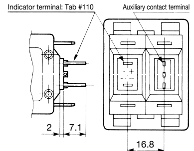
Illuminated Rocker (2-pole) Relay Trip (4-terminal)
